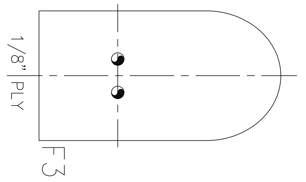
SECTION 4 SCALE FULL
