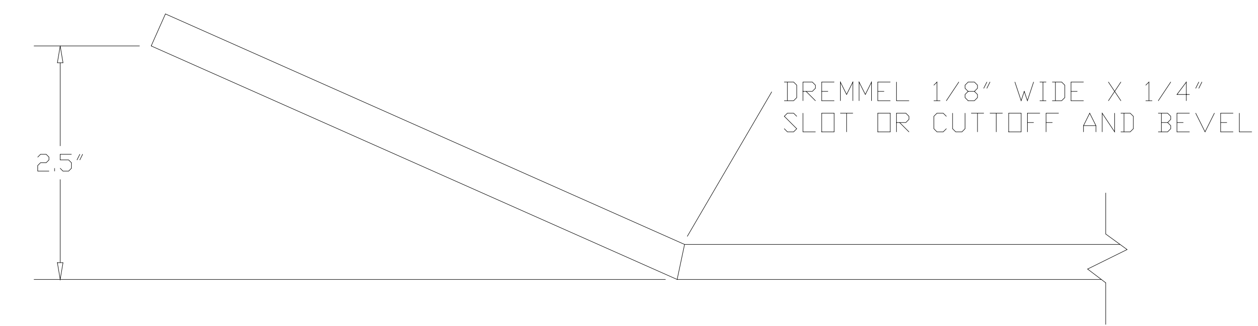
SECTION "A-A"
