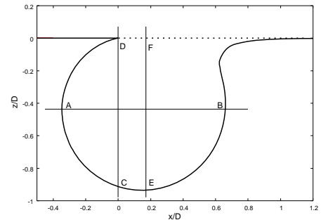
Fig. 3 Cavity cell
