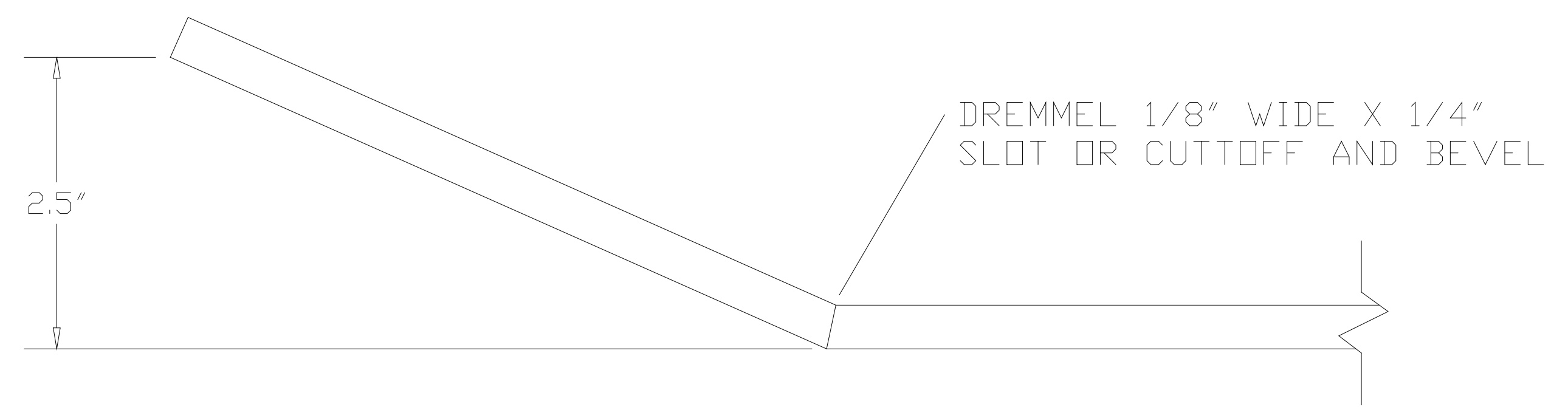
SECTION "A-A"
